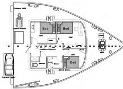
SECOND LEVEL SCALE 1:75
