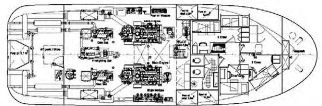
Below Maindeck
